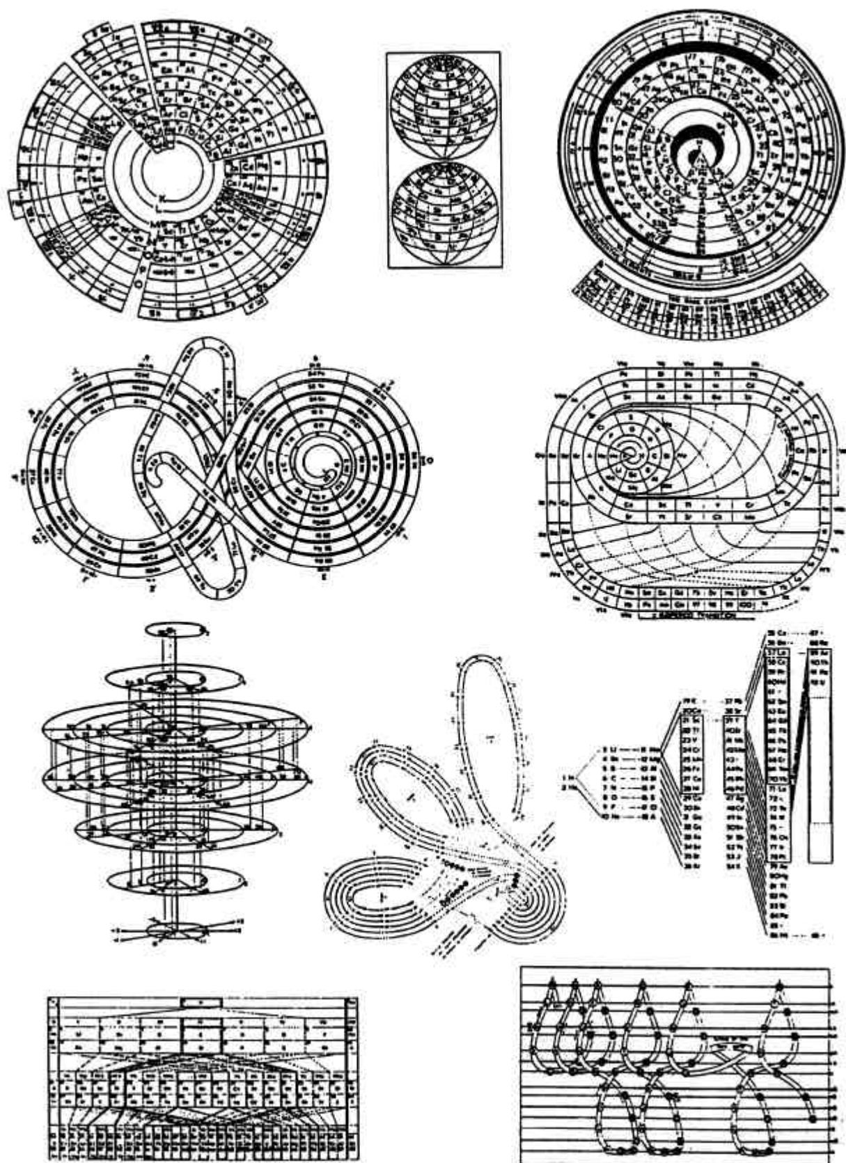
Figure 2. Examples of past attempts to present the periodic classification of chemical elements (Reproduced from J W van Spronsen, The Periodic System of Chemical Elements)
