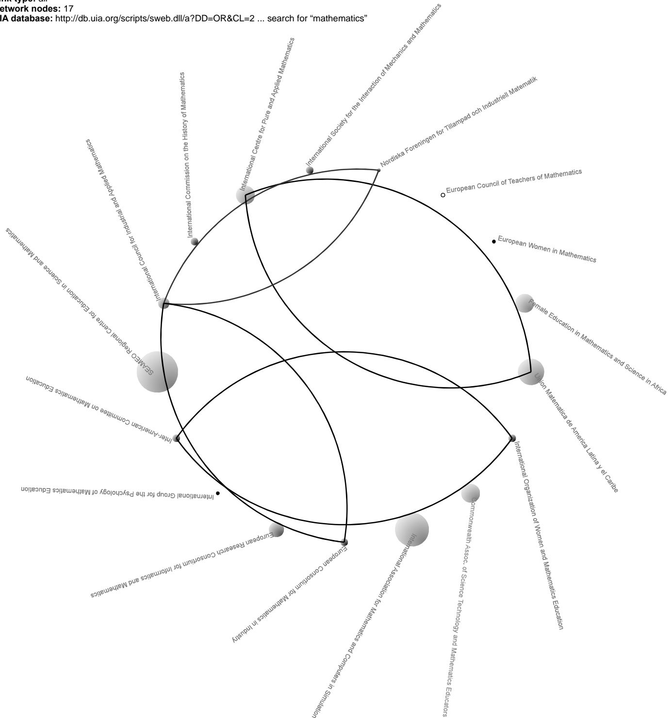
Figure 10.1.12. Relations amongst international organizations concerned with mathematics (A-F)
