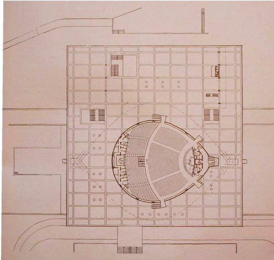
AUDITORIUM PLAN
